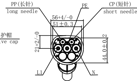
16A桩端插头5POS 16A pile end plug 5POS
