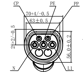
16A车辆端插头5POS 16A Vehicle end plug 5pos
