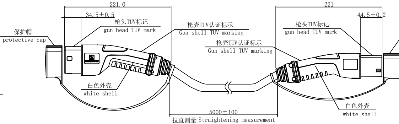
16A车辆端插头5POS 16A Vehicle end plug 5pos
