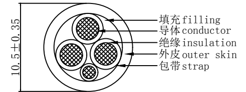
充电枪线缆: 3X2.5mm 2 +1X0.5mm 2 黑色外皮 Charging gun cable: 3X2.5mm 2 +1X0.5mm 2 black
