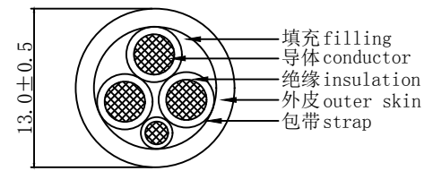
充电枪线缆: 3X6 2 +1X0.5mm 2 黑色外皮 Charging gun cable: 3X6mm 2 +1X0.5mm 2 black
