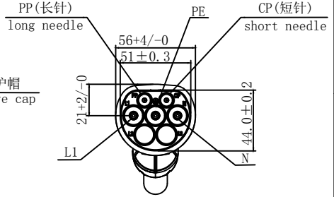
32A桩端插头5POS 32A pile end plug 5POS
