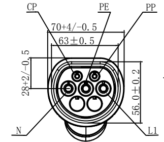
32A车辆端插头5POS 32A Vehicle end plug 5pos
